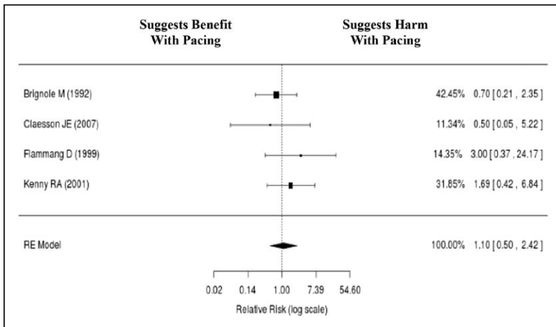
Figure 3. Forest Plot of Meta-Analysis of Mortality Rate.
