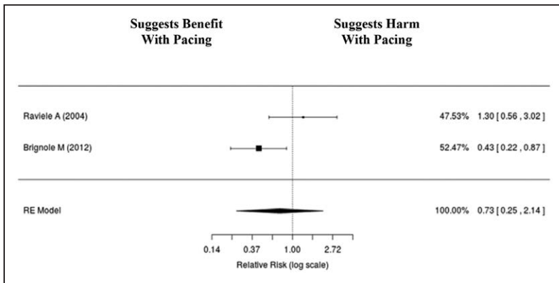
Figure 2B. Forest Plot of Meta-Analysis of Recurrent Syncope (Double-Blinded Studies).
