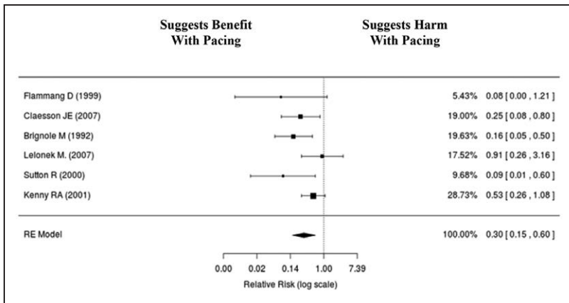
Figure 2A. Forest Plot of Meta-Analysis of Recurrent Syncope (Unblinded Studies).
