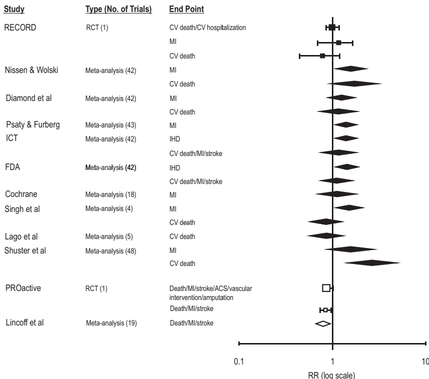
Figure. Thiazolidinediones and IHD risk based on randomized controlled trials (closed and open squares) and their meta-analyses (closed and open diamonds). Data for rosiglitazone are shown as closed squares and diamonds, whereas data for pioglitazone are shown as open squares and diamonds. There is overlap among the individual studies included in the different meta-analyses. RCT indicates randomized, controlled trial; CV, cardiovascular; ICT, integrated clinical trial; and ACS, acute coronary syndrome.
