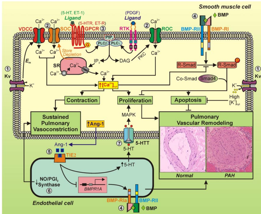
Figure 1. Schematic depicting the potential “hits” involved in the development of PAH. A rise in [Ca^{2+}]_{cyt} in PASMCS (due to decreased Kv channel activity ① and membrane depolarization, which opens VDCCs; upregulated TRPC channels that participate in forming receptor- and store-operated Ca^{2+} channels ②; and upregulated membrane receptors [e.g., serotonin, endothelin, or leukotriene receptors] ③; and their downstream signaling cascades) causes pulmonary vasoconstriction, stimulates PASM proliferation, and inhibits the BMP-signaling pathway that leads to antiproliferative and proapoptotic effects on PASMCS. Dysfunction of BMP signaling due to BMP-RII mutation and BMP-RII/BMP-RI downregulation ④ and inhibition of Kv channel function and expression ① attenuate PASM apoptosis and promote PASM proliferation. Increased Ang-1 synthesis and release ⑤ from PASMCS enhance 5-HT production and downregulate BMP-RIA in PAECs and further enhance PASM contraction and proliferation, whereas inhibited nitric oxide and prostacyclin synthesis ⑥ in PAECs would attenuate the endothelium-derived relaxing effect on pulmonary arteries and promote sustained vasoconstriction and PASM proliferation. Increased activity and expression of the 5-HTT ⑦ would serve as an additional pathway to stimulate PASM growth via the MAPK pathway. In addition, a variety of splicing factors, transcription factors, protein kinases, extracellular metalloproteinases, and circulating growth factors would serve as the “hits” to mediate the phenotypical transition of normal cells to contractive or hypertrophied cells and to maintain the progression of PAH.
